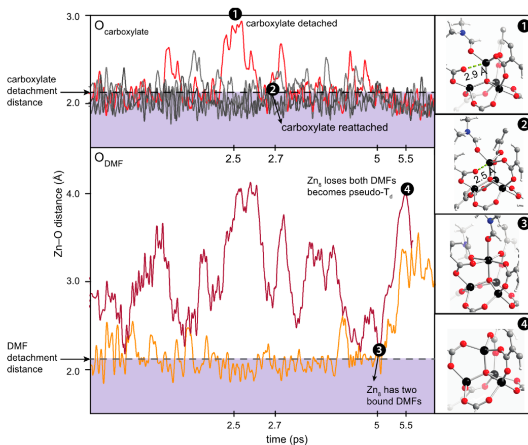
Figure 4. Summary of the BOMD simulated trajectories corresponding to the pseudo-octahedral Zn site, Zn_8 , for the first 6 ps. Zn–O distances are plotted at the top for the framework carboxylates and at the bottom for the two nearest DMF molecules. Snapshots of the simulation are shown at time points (ps) on the right. The carboxylate oxygen that dissociates completely is shown as the red trace in the O_{\text{carboxylate}} panel. The two colored traces in the O_{\text{DMF}} panel represent the positions of the oxygen atoms of two DMF molecules in the vicinity of Zn_8 . The Zn–O bonding regions are defined by the colored rectangular regions starting at 2.2 Å for both carboxylate and DMF oxygen atoms.
