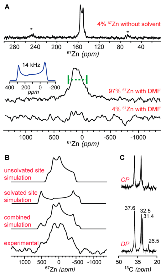
Figure 2. (A) ^{67}\text{Zn} NMR spectra of MOF-5 taken under magic-angle spinning conditions at 21.1 T: fully evacuated (top) and when solvated with DMF using enriched (middle) and natural abundant (bottom) zinc. Asterisks denote spinning side bands. The spectral inset (blue) illustrates the secondary site present within the solvated system. (B) ^{67}\text{Zn} nonspinning NMR spectra of experimental 97% enriched sample soaked in DMF alongside spectra for two simulated sites collected at 11.7 T. (C) ^{13}\text{C} MAS NMR spectra taken of \text{CH}_2\text{Cl}_2 - and DMF-soaked MOF-5 with only the methyl region displayed using direct-polarization (DP) and ^{13}\text{C}[^1\text{H}] cross-polarization (CP).
