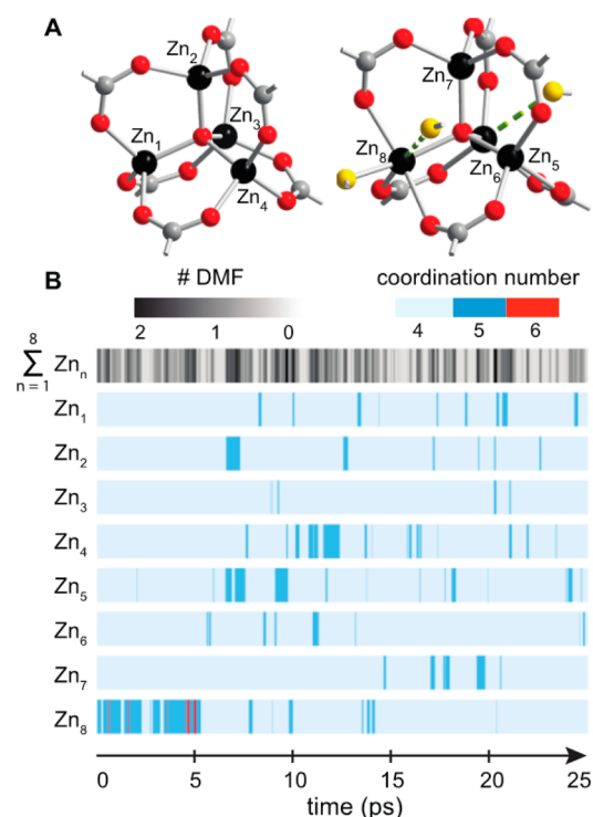
Figure 3. (A) Cluster 1 (left) and cluster 2 (right) of the two \text{Zn}_4(\mu_4\text{-O})(1,4\text{-benzenedicarboxylate})_3 units employed for the simulation as they appear at time = 0 ps. Carbonyl oxygen atoms from DMF solvent are depicted in yellow. (B) Coordination number for individual Zn sites ( \text{Zn}_1 through \text{Zn}_8 ) along the BOMD 25 ps simulation. Light blue denotes a coordination number of 4, dark blue 5, and red 6. The total number of DMF molecules bound to any of the eight Zn sites, \text{Zn}_1 through \text{Zn}_8 , is shown at the top on a spectrum from zero to two, denoted by white to black, respectively.
